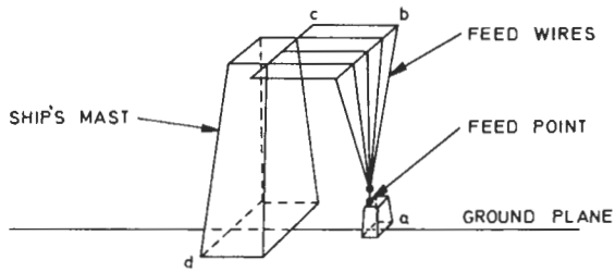
FOLDED MONOPOLE AERIAL
