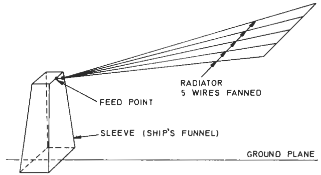
MODIFIED SLEEVE AERIAL
