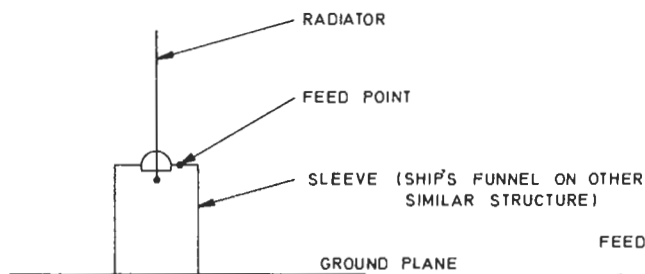
SLEEVE AERIAL
