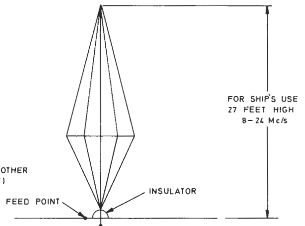
BICONICAL (MONOPOLE) AERIAL
